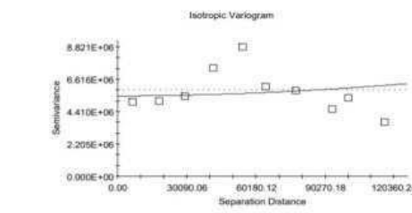
Gaussian model (Co = 5480000.0000; Co + C = 10961000.0000; Ao = 311000.00; r2 = 0.208; RSS = 2.248E+13)
