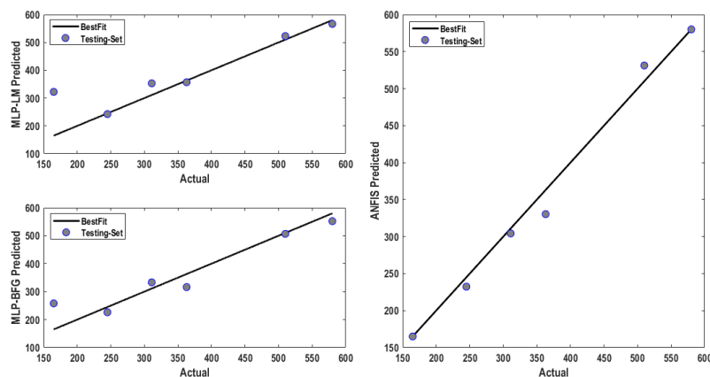
Figure 6. The distribution of estimates of groundwater quality variables and their actual values for the TDS variable
