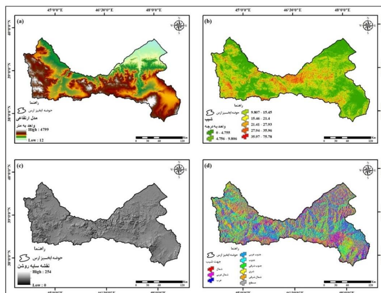
Figure 4. a: Elevation model map, b: Slope Map, c: Bright Shadow map, d: Slope direction map (Authors, 2023)
