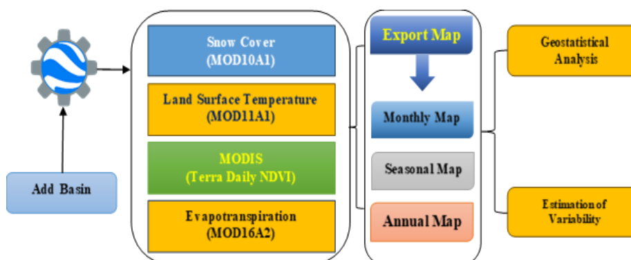
Figure 3. Products and maps used in the research (Authors, 2023)
