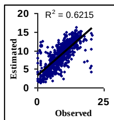
Figure 5. Q-Q plot of optimal ANFIS model with 4 input variables
