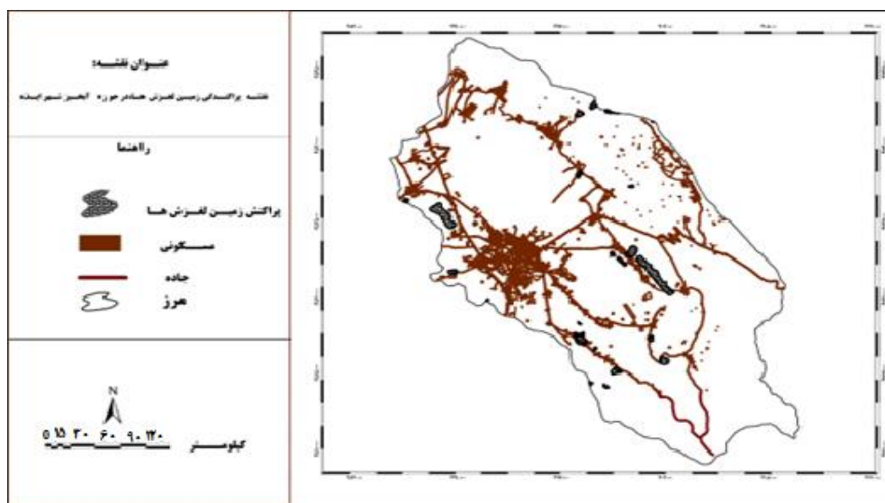
Figure 5. The spatial distribution map of landslides Izeh watershed (source authors)
